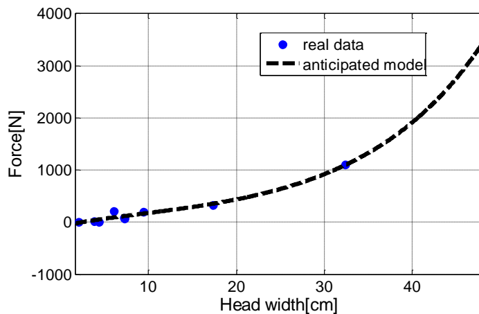
Figure 6. Graph illustrating the scaling of bite force relative to head width
