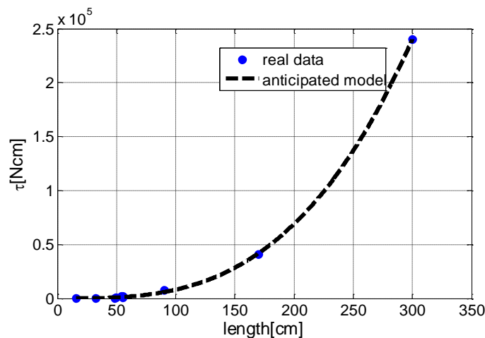
Fig. 8. Graph illustrating relationship between torque and length
