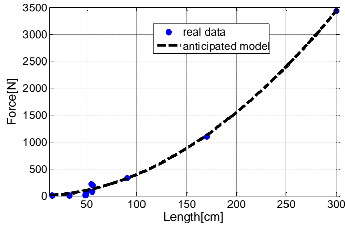
Figure 4. Graph illustrating the scaling of bite force relative to length
